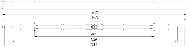
в) Trade Linear 1472x65x60
