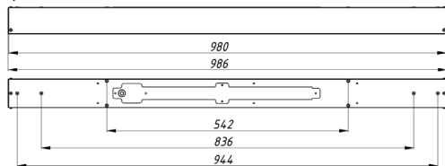
b) Trade Linear 980x65x60
