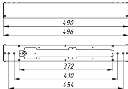
a) Trade Linear 490x65x60
